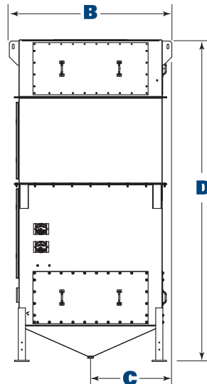
Side View ADMC-AD6
